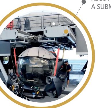
LAUNCH AND RECOVERY SYSTEM FOR A SUBMARINE ABS SWL 14
