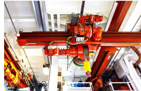
CRANES FOR LOAD HANDLING BETWEEN DECKS AND LABORATORIES.
